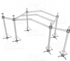
12D PR3 Stage Roofing System with 7 Ft Speaker Wings and 6 Chain Hoists | 30 Ft W x 20 Ft L x 23 Ft H SKU: XTP-GS302023-PR3-12D
