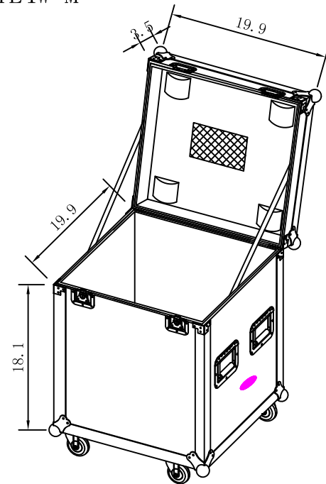
XS-UTL4W-M
